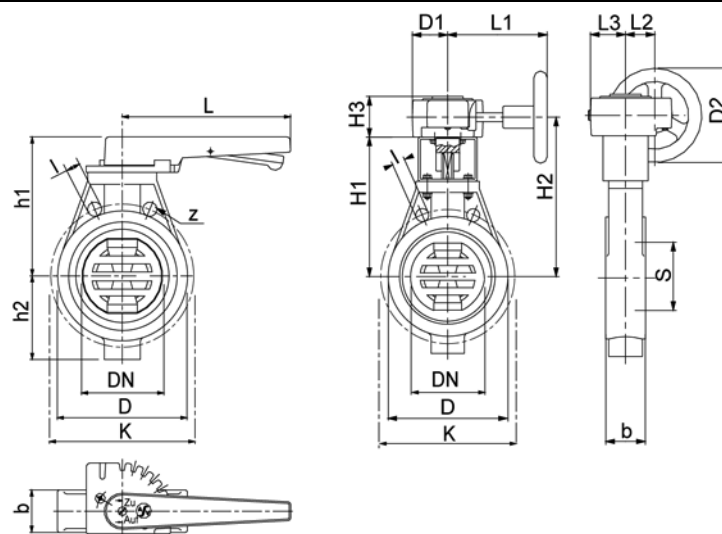
DN 50 - DN 200
